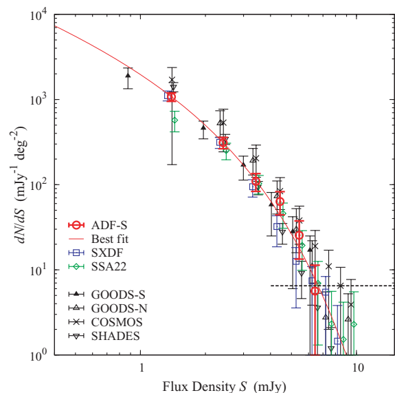
Figure 7. Differential number counts in the ADF-S, the SXDF and the SSA 22 fields surveyed by AzTEC/ASTE. The counts are calculated for the 50 per cent coverage regions. The error bars represent the 68.3 per cent confidence intervals. The red curve represents the best-fitting Schechter functional form of the ADF-S: dN/dS = N_{3\text{mJy}}(S/3\text{mJy})^{-1} \exp(-(S - 3\text{mJy})/S') with N_{3\text{mJy}} = 169 \pm 19 and S' = 1.48 \pm 0.20 . The number counts of previous 1.1-mm surveys are also shown: GOODS-N (Perera et al. 2008), COSMOS (Austermann et al. 2009), SHADES (Austermann et al. 2010) and GOODS-S (Scott et al. 2010). The horizontal dashed line represents the survey limit of the ADF-S, which Poisson deviations to zero sources per bin 32.7 per cent. The bin centres of some number counts are shifted by \pm 3 per cent for easier comparison.
