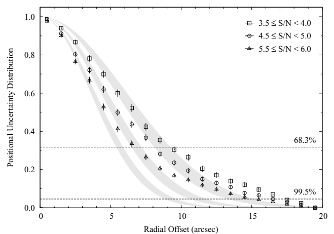
Figure 6. Probability that a source is detected outside an angular distance from its true position. The probability is calculated for sources with 3.5 \leq S/N < 4.0 , 4.5 \leq S/N < 5.0 and 5.5 \leq S/N < 6.0 . The horizontal dashed lines indicate 68.3 and 99.5 per cent confidence intervals. The shaded regions represent theoretical predictions derived in Ivison et al. (2007) for the S/N ranges.
