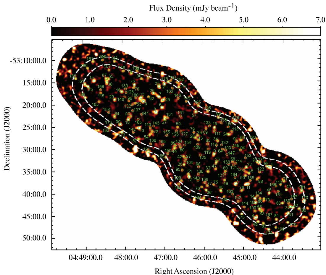
Figure 1. Signal map of the ADF-S. White contours represent the 30 per cent (outer contour) and 50 per cent (inner contour) coverage regions (corresponding to rms noise levels of 0.55 and 0.71 mJy beam -1 ), respectively. The 198 sources detected with \geq 3.5\sigma in the 30 per cent coverage region are indicated by green circles with a 30-arcsec diameter and numbered in order of significance (Table 2). The pixel size is 3 \times 3 arcsec 2 .
