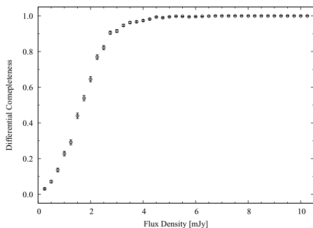
Figure 5. Survey completeness for the 50 per cent coverage region. The error bars are 1\sigma from the binomial distribution.
