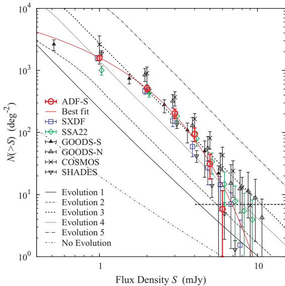
Figure 9. Comparison of 1.1-mm observed number counts with the models of Takeuchi et al. (2001b). Descriptions of the models are in Section 5.4.
