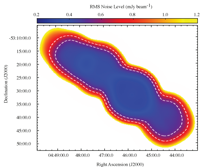
Figure 2. Noise map of the AzTEC/ASTE ADF-S. The outer and inner contours indicate the 30 and 50 per cent coverage regions, respectively.
