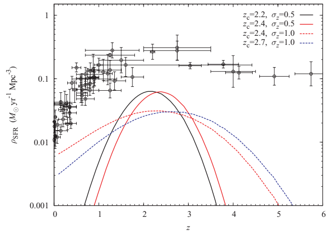
Figure 12. SFR density estimated from the best-fitting number counts in the ADF-S. Four redshift distributions are assumed. The SFR densities are calculated by integrating the number counts at \geq 1 mJy and using the SED model of Arp 220. The results from previous UV/optical observations are plotted for comparison (compiled data are taken from Hopkins 2004, and references therein).
