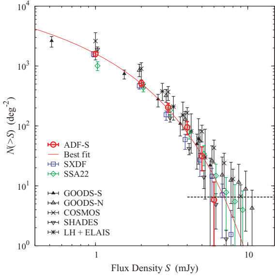
Figure 8. Cumulative number counts in the ADF-S, the SXDF and the SSA 22 fields surveyed by AzTEC/ASTE. The counts are calculated for the 50 per cent coverage regions. The error bars indicate 68.3 per cent confidence intervals. The red curve represents the best-fitting Schechter functional form of the ADF-S. Number counts of previous 1-mm surveys are also shown: the AzTEC/JCMT surveys of GOODS-N (Perera et al. 2008), COSMOS (Austermann et al. 2009), SHADES (Austermann et al. 2010), the AzTEC/ASTE GOODS-S (Scott et al. 2010), 1.2-mm MAMBO surveys of the Lockman Hole and ELAIS N2 regions (Greve et al. 2004). The horizontal dashed line represents the survey limit of the ADF-S, which Poisson deviations to zero sources per bin 32.7 per cent. The bin centres of some number counts are shifted by \pm 3 per cent for easier comparison.
