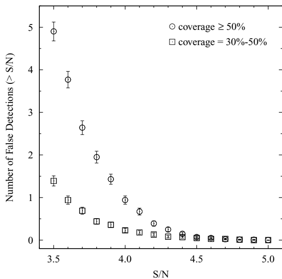
Figure 4. Number of false detections expected above given signal-to-noise ratio thresholds calculated in the 50 and 30–50 per cent coverage regions. The error bars are 1\sigma Poisson uncertainties.
