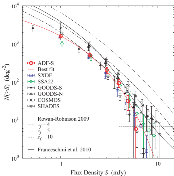
Figure 10. Comparison of 1.1-mm observed number counts with the models of Rowan-Robinson (2009) and Franceschini et al. (2010). Descriptions of the models are in Section 5.4.
