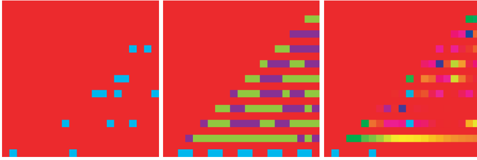
Figure 5. \Delta\Phi_{\ell m} for Bianchi types V (left), \text{VII}_0 (middle) and \text{VII}_h (right) where \ell, m \in [0, 20] and z = 0 . Note that \ell is plotted against the x axis, increasing from left to right, and m is plotted against the y axis, increasing from bottom to top. Like the phases (Fig. 4) the distributions are not random but exhibit some distinctive features. All the \Delta\Phi_{\ell m} for the V type are either 0 or \pi . The \Delta\Phi_{\ell m} for the \text{VII}_0 type are again orthogonal but in a more correlated way. Similarly, the sequences of colours in the type \text{VII}_h are now even more prominent (see m = 2 ).
