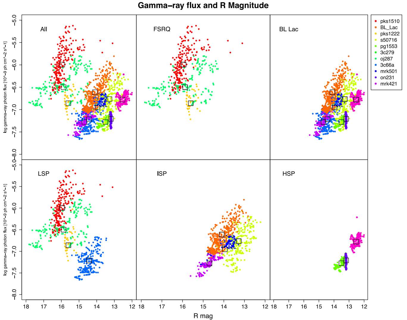
Figure 2. Fermi \gamma -ray data plotted against magnitude for 11/15 sources (those which have >5 \gamma -ray data points) (each with a separate colour) and subsequent blazar subclasses: FSRQs, BL Lacs, LSPs, ISPs and HSPs. The \gamma -ray data points are interpolated to match the date of the optical data points (see Section 4.1). Black squares show the mean \gamma -ray and optical value for each source.
