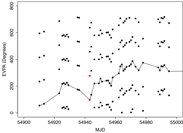
Figure 1. Zoomed view of PKS 1510-089 light curve (full light curve shown in appendix, Fig. A2). This plot can be compared with fig. 4 in Marscher et al. (2010) where the polarization angle data are interpreted as showing a 720^\circ rotation. Here we report a rotation of less than half that ( 333^\circ ) and this is due to the interpretation of this particular data set by the EVPA trace code which, to account for the \pm 180 , ambiguity identifies the next nearest lying point. The points in red highlight where the difference in identification originates.
