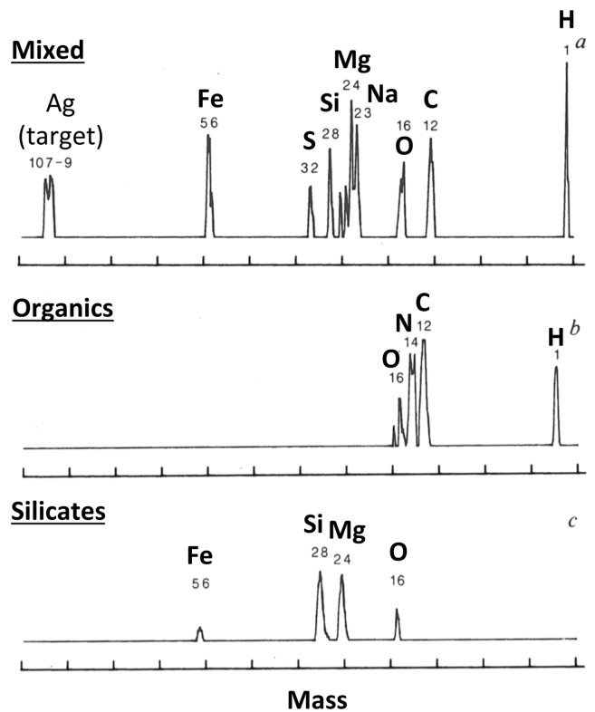
Figure 1. Typical mass spectra obtained by the PIA instrument (particle impact analyser), a mass spectrometer on the Giotto spacecraft (vertical log scale) (adapted from Kissel et al. 1986a). Proposed element identification has been added to the mass peaks for clarity. The mixed (a) and organics (b) types represent 80 per cent of the total number of spectra (see original article for details). Reprinted by permission from Macmillan Publishers Ltd: Nature, copyright (1986).
