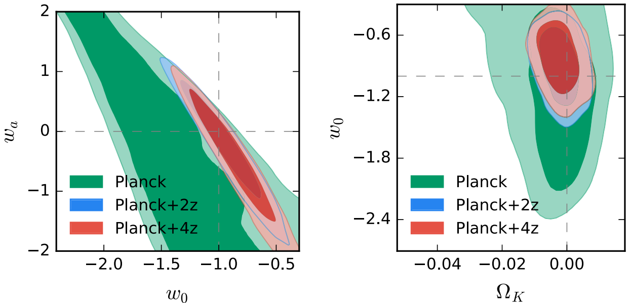
Figure 6. Left panel: 2D marginalized contours for 68 per cent and 95 per cent confidence level for w_0 and w_a ( w_0w_a CDM model assumed) from Planck -only (green), Planck +CMASS (one bin)+LOWZ (one bin) (blue), and Planck +CMASS (two bins)+LOWZ (two bins) (red); right panel: 2D marginalized contours for 68 per cent and 95 per cent confidence level for \Omega_K and w_0 ( ow_0w_a CDM model assumed). One can see that w_0 and w_a are consistent with -1 and 0 , respectively, which correspond to the \Lambda CDM.
