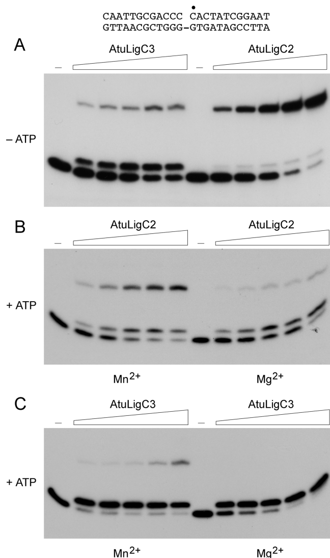
Figure 2. Nick-sealing activity of AtuLigC2 and AtuLigC3. (A) Reaction mixtures (20 \mu l) containing either 50 mM Tris-HCl (pH 7.5) (AtuLigC2) or 50 mM Tris-acetate (pH 6.0) (AtuLigC3), 5 mM DTT, 5 mM MnCl_2 , 1 pmol ^{32}P -labeled nicked 24-mer DNA substrate (depicted at the top with the labeled 5' nucleotide at the nick indicated by filled circle), and increasing amounts of AtuLigC2 (38, 75, 150, 300 and 600 ng) or AtuLigC3 (50, 100, 200, 400 and 800 ng) were incubated for 20 min at 37°C. Enzyme was omitted from a control reaction mixture (lane -). The products were resolved by PAGE and visualized by autoradiography. (B) Reaction mixtures (20 \mu l) containing 50 mM Tris-HCl (pH 7.5), 5 mM DTT, 5 mM MnCl_2 (left panel) or 5 mM MgCl_2 (right panel), 250 \mu M ATP, 1 pmol ^{32}P -labeled nicked 24-mer DNA substrate, and increasing amounts of AtuLigC2 (38, 75, 150, 300 and 600 ng) were incubated at 37°C for 20 min. Enzyme was omitted from a control reaction mixture (lane -). (C) Reaction mixtures (20 \mu l) containing 50 mM Tris-acetate (pH 6.0), 5 mM DTT, 5 mM MnCl_2 (left panel) or MgCl_2 (right panel), 250 \mu M ATP, 1 pmol ^{32}P -labeled nicked 24-mer DNA substrate, and increasing amounts of AtuLigC3 (50, 100, 200, 400 and 800 ng) were incubated at 37°C for 20 min. Enzyme was omitted from a control reaction mixture (lane -).
