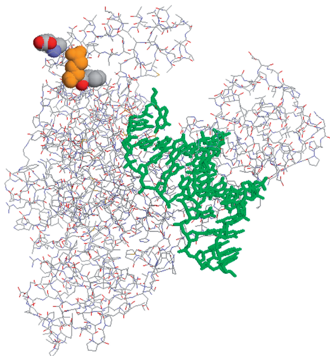
Figure 9. Location of the mutagenized codons in KlenTaq. Crystal structure from pdb file 2KTQ (51) emphasizes the location of the residues mutated in KlenTaq 10. Using full-length Taq numbering, w.t. residues are rendered in spacefill for the mutated positions 626 707 (C5-mutations), and 708 (orange, blood and soil-resistance mutation) using the program Rasmol 2.7.1 (53). Upper right is the thumb domain, upper left is the fingers domain, where the mutations can be seen at the surface of the hinge point (knuckles) of the fingers. Primer and template DNA strands are rendered in stick mode (green) in the active site cleft.
