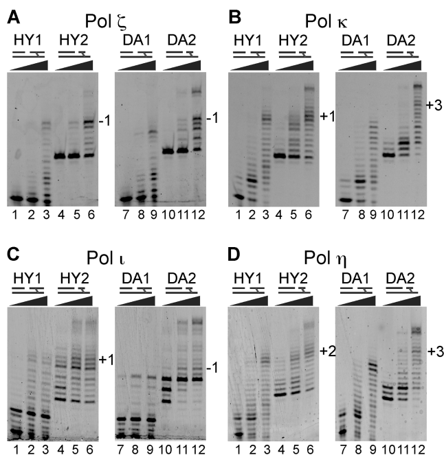
Figure 5. Resected NML ICLs can be bypassed by multiple Y-family polymerases. Full-length (HY1, DA1) and 5'- and 3'-resected (HY2, DA2) NML templates were annealed to primers P15 and P7, respectively, and incubated with increasing concentrations of (A) Pol \zeta (0.4, 4, 35 nM), (B) Pol \kappa (0.2, 2, 20 nM), (C) Pol \iota (4, 40, 400 nM) and (D) Pol \eta (4, 40, 400 nM). The position of the main stalling points is indicated at the right side of the gels. Note the marked presence of full length products indicated.
