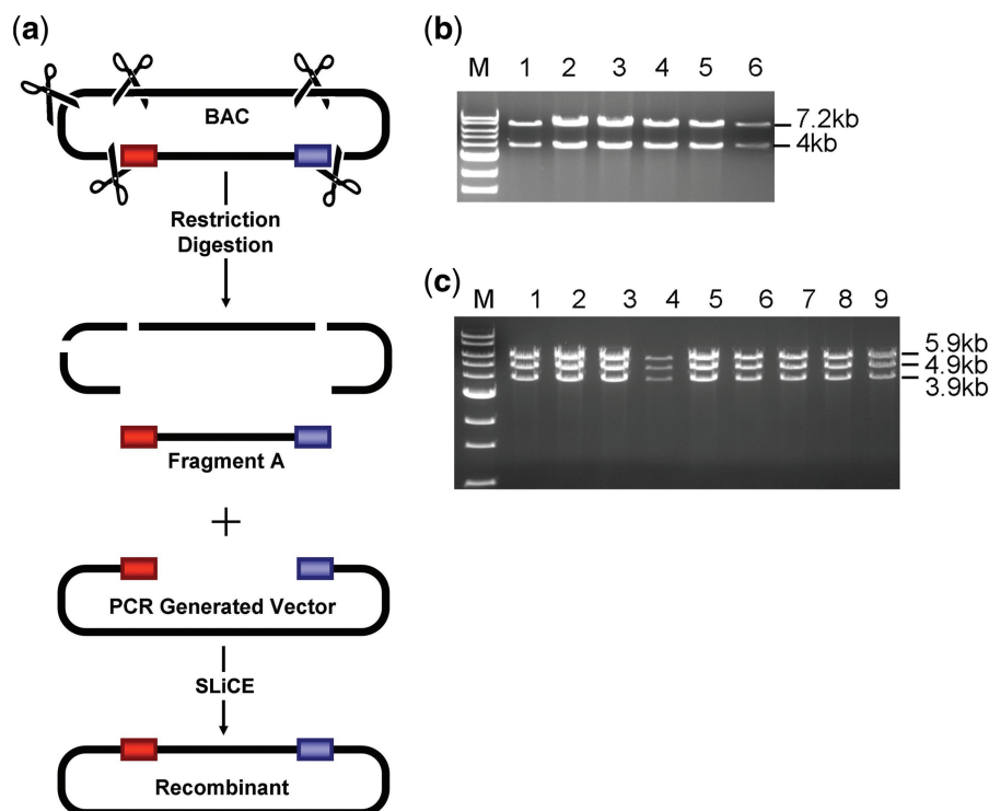
Figure 3. BAC SLiCE Cloning. (a) Schematic illustrating BAC SLiCE cloning. (b) XmnI/XhoI restriction analysis of recombinants derived from SLiCE cloning of an 8.7-kb BglIII BAC fragment. Plasmid DNAs from six independent ampicillin-resistant colonies (lanes 1–6) were digested with XmnI and XhoI. Recombinants contain one XmnI site within the vector and one XhoI site within the insert yielding diagnostic 7.2- and 4-kb restriction fragments. (c) BamHI/BglIII restriction analysis of recombinants derived from SLiCE cloning of a 12.2-kb EcoRV BAC fragment. Plasmid DNAs from nine independent ampicillin-resistant colonies (lanes 1–9) were digested with BamHI and BglIII. Recombinants contain one BglIII site within the vector and two BamHI sites in the insert yielding diagnostic 5.9-, 4.9- and 3.9-kb restriction fragments.
