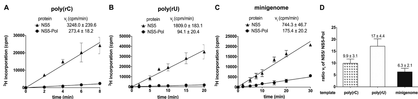
Figure 1. NS5 and NS5-Pol activity on homopolymeric and heteropolymeric templates analyzed by filter binding. Reactions kinetics were determined as given in Materials and Methods (RdRp assay 1). Reactions were done in HEPES reaction buffer with (A) 100 nM poly(rC), 40 nM protein, 20 \mu M GTP, (B) 100 nM poly(rU), 100 nM protein, 200 \mu M ATP, (C) 100 nM minigenome, 100 nM protein, 300 \mu M ATP, CTP, GTP, 4 \mu M UTP. Incorporation of 3 H-labeled NTPs was measured in counts per minute (cpm). (D) Ratios of NS5 and NS5-Pol activities are given for different RNA templates. The tests were done in triplicates.
