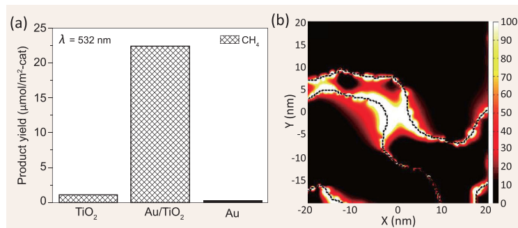
Figure 5. (a) Photocatalytic product yields (after 15 h of visible-light irradiation) on three different catalytic surfaces. (b) Electric-field intensity at the interface of \text{Au}-\text{TiO}_2 to \text{CH}_4 under UV-vis irradiation [66]. It was found that \text{AuPt}/\text{TiO}_2 exhibited a 1.8-fold and 1.4-fold higher \text{CH}_4 production compared to \text{Au}/\text{TiO}_2 and \text{Pt}/\text{TiO}_2 , respectively. The higher activity was attributed to the improved charge-carrier separation induced by the LSPR effect of \text{Au} and the \text{Pt} NPs as electron sinks and reduction sites. In addition to the enhancement effect, LSPR was also demonstrated to modulate the selectivity in \text{CO}_2 photoreduction. Reduced graphene-coated \text{Au} NP ( r\text{-GO-AuNPs} )- \text{TiO}_2 hybrid photocatalysts were demonstrated to effectively convert \text{CO}_2 into \text{HCOOH} [67]. The hybrid material (quantum yield: 1.52%) showed excellent selectivity for \text{HCOOH} (>90%) and higher conversion efficiency than \text{Pt} -coated \text{Au} NPs- \text{TiO}_2 hybrid material (quantum yield: 1.14%). Zhou and Zou et al. prepared an \text{Au}@\text{TiO}_2 yolk-shell hollow sphere [68]. An LSPR-mediated electromagnetic field near to \text{Au} nanoparticles is claimed not only to enhance the local generation and subsequent separation of e^-h^+ pairs in \text{TiO}_2 shells to improve the yield of photoreduction \text{CO}_2 , but also to facilitate chemical reactions involving multiple e^-/h^+ transfer processes to allow the formation of high-quality carbon species ( \text{C}_2\text{H}_6 ), which was rarely observed in present \text{CO}_2 photocatalytic-reduction systems. These results provide a novel way in developing efficient MSC materials for \text{CO}_2 photoreduction, which could inspire future work in this area.
