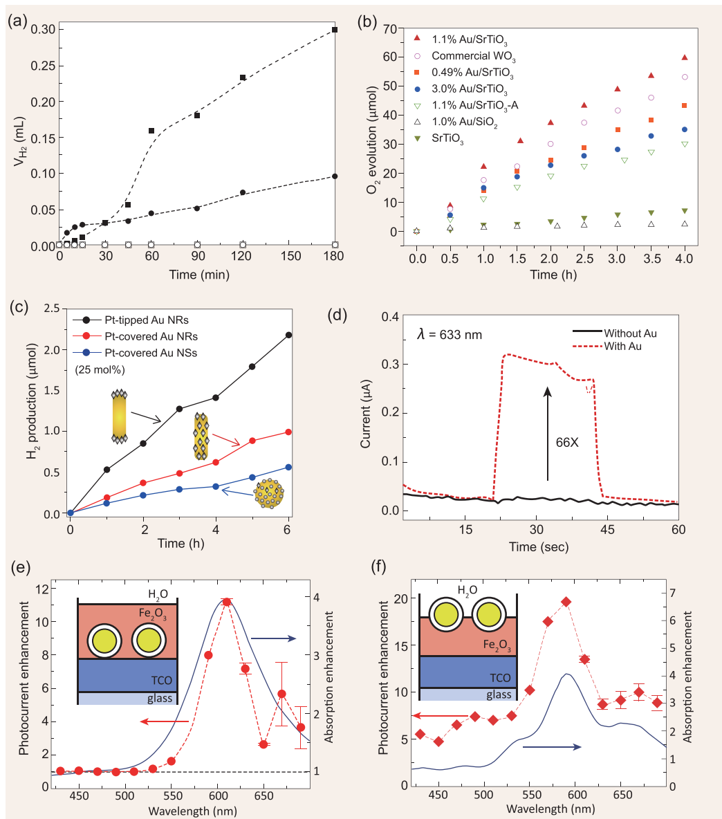
Figure 4. (a) Volume of hydrogen evolved during the photocatalytic runs using \text{TiO}_2 and Au (1.5 wt %)/ \text{TiO}_2 as catalysts and Ethylenediaminetetraacetic acid (EDTA) as sacrificial electron donor, under 532-nm laser irradiation and polychromatic light \lambda > 400 nm. ■: Au/ \text{TiO}_2 , \lambda = 532 nm; •: Au/ \text{TiO}_2 , \lambda > 400 nm; ○: \text{TiO}_2 , \lambda = 532 nm; □: \text{TiO}_2 , \lambda > 400 nm [49]. Reprinted with permission from Ref. [49]. Copyright 2011, by the American Chemical Society. (b) Curves of \text{O}_2 evolution as a function of reaction time under visible-light irradiation ( \lambda > 400 nm). Reaction conditions: 0.2 g catalyst, 5 mmol \text{AgNO}_3 , 300-W Xe lamp [20]. Adapted with permission. Copyright 2014, by The Royal Society of Chemistry. (c) Time course of \text{H}_2 evolution from water–methanol (20 vol %) suspensions of Pt-modified Au NPs (0.188 mg) under visible-light irradiation ( 460 < \lambda < 820 nm) [53]. Reprinted with permission from Ref. [53]. Copyright 2014, by the American Chemical Society. (d) Photocurrent of anodic \text{TiO}_2 with and without Au NPs irradiated with \lambda = 633 nm light for 22 s [56]. Reprinted with permission from Ref. [56]. Copyright 2011, by the American Chemical Society. (e, f) Photocurrent enhancement spectra for Au NPs with a silica shell. Measured photocurrent (red symbols) and simulated (solid blue lines) absorption enhancement spectra that show the beneficial effects of placing silica-coated Au NPs at the bottom (e)/on top (f) of a 100-nm thin \text{Fe}_2\text{O}_3 photoelectrode layer [30]. Reprinted with permission from Ref. [30]. Copyright 2011, by the American Chemical Society.
