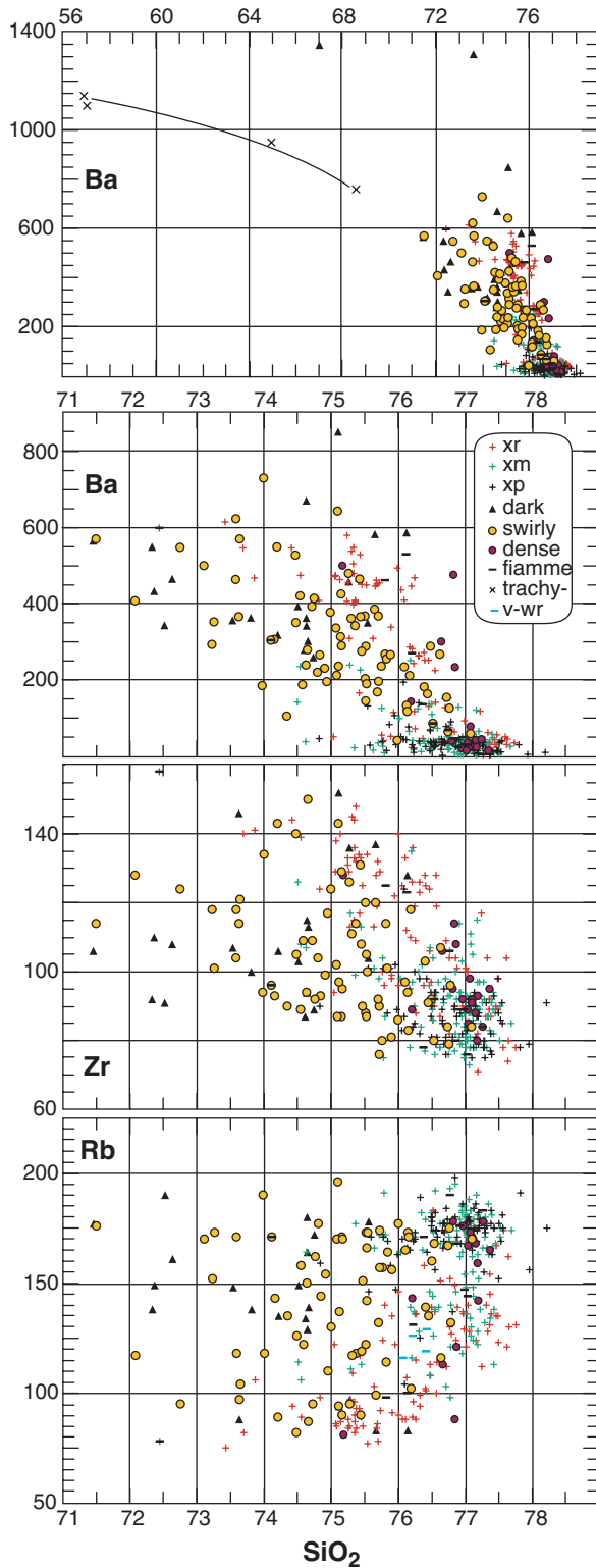
Fig. 10. Ba, Zr, and Rb (in ppm) vs wt % SiO 2 for pumice clasts in the Bishop Tuff. Clast types identified in inset, as in Fig. 9; also plotted are four whole-rock welded-tuff vitrophyre samples (v-wr). The top panel is extended as in Fig. 9 to include the rare trachy-andesites and dacites (curved tie-line).
