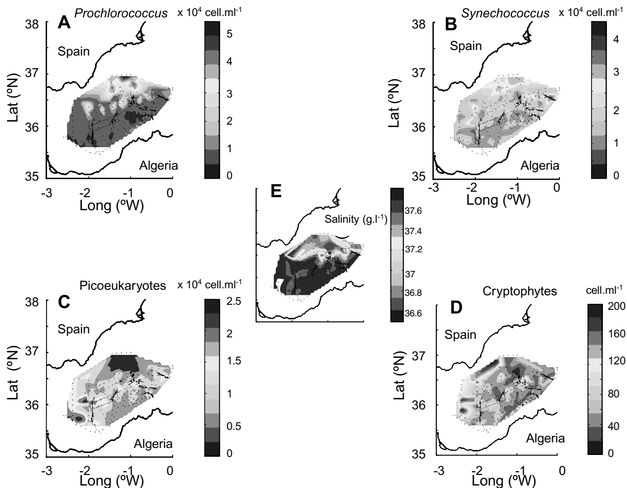
Fig. 4. Maps of cell abundance for Prochlorococcus (A), Synechococcus (B), picoeukaryotes (C), cryptophytes (D) and of salinity (E) in surface waters of the Alboran Sea between December 24, 1997 and January 9, 1998.
