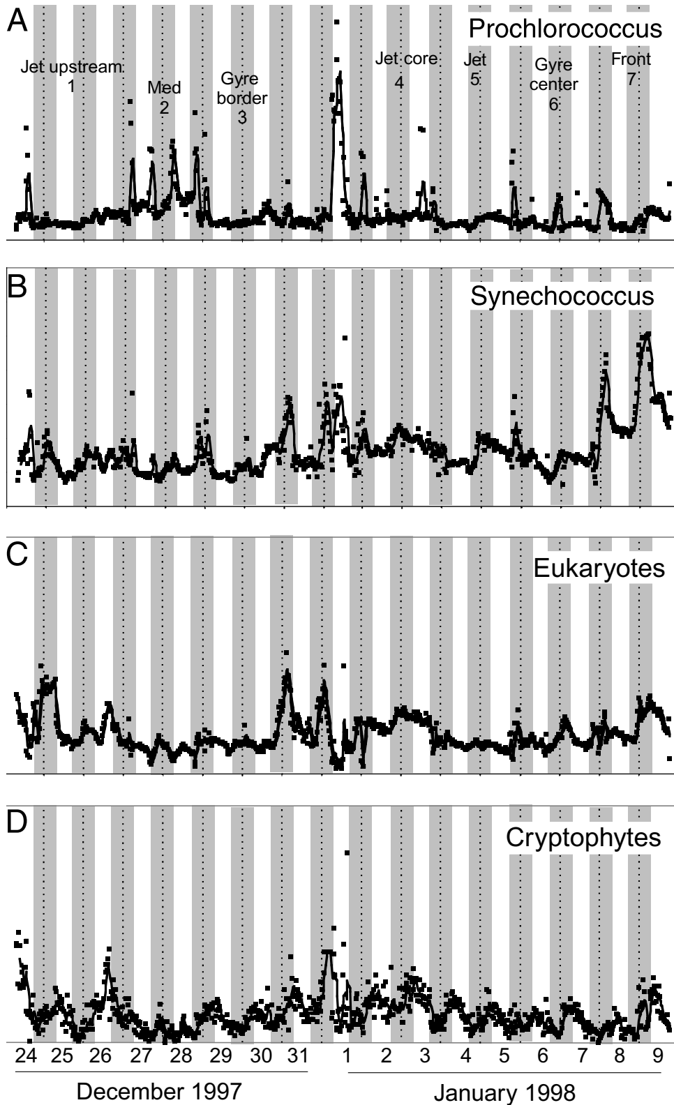
Fig. 5. Cell abundance of Prochlorococcus (A), Synechococcus (B), picoeukaryotes (C) and cryptophytes (D) in surface waters of the Alboran Sea sampled every 30 min between December 24, 1997 and January 9, 1998. Curves fitting the data correspond to a third-order moving average. Vertical grey bars symbolize periods of darkness.
