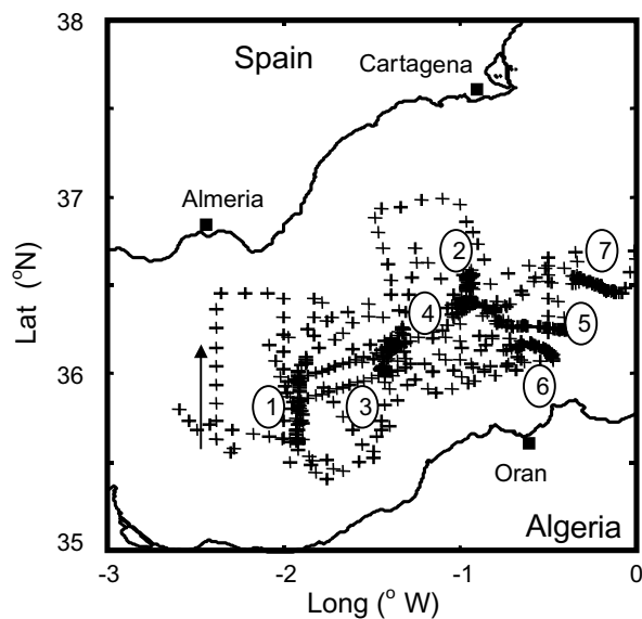
Fig. 1. The Alboran Sea with 30 min interval sampling locations during this study symbolized by +. Sites correspond to well-defined hydrological situations, i.e. 'Mediterranean waters' (site 2), the Atlantic baroclinic jet (sites 1, 4, 5), the Almeria-Oran front (site 7) and the eastern Alboran gyre (sites 3, 6). The arrow indicates the beginning and the direction of sampling.
