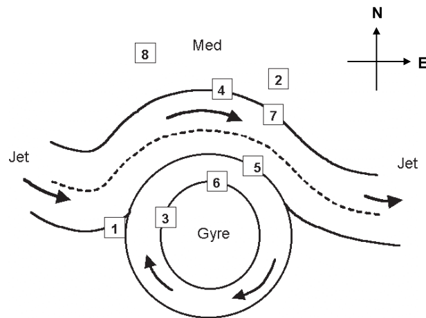
Fig. 2. Schematic positions of sites in the jet-front-gyre system explored during leg-2 of the cruise.
