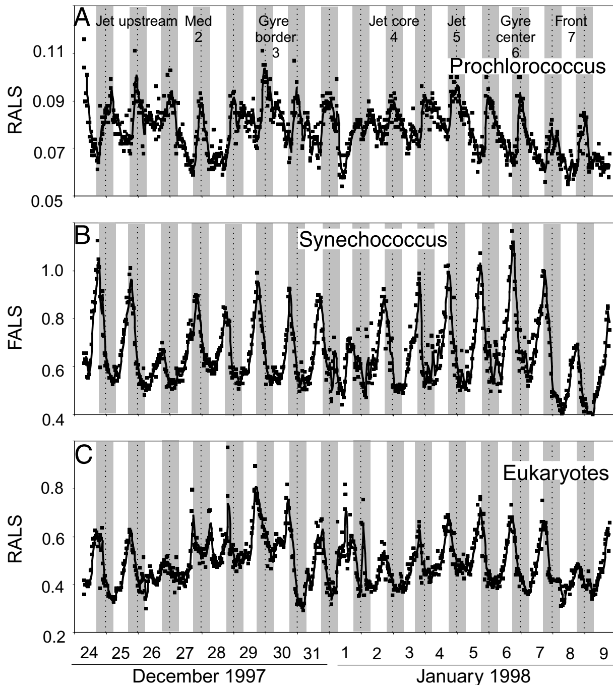
Fig. 6. Light scatter (RALS or FALS) of Prochlorococcus (A), Synechococcus (B) and picoeukaryotes (C) sampled every 30 min between December 24, 1997 and January 9, 1998. Curves and symbols as on Figure 5.
