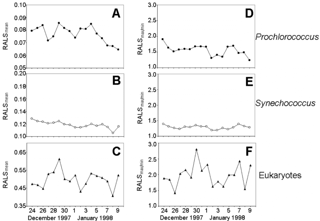
Fig. 7. Daily mean value of RALS and of the RALS max/min ratio for Prochlorococcus (A, D), Synechococcus (B, E) and picoeukaryotic cells (C, F) between December 24, 1997 and January 9, 1998.
