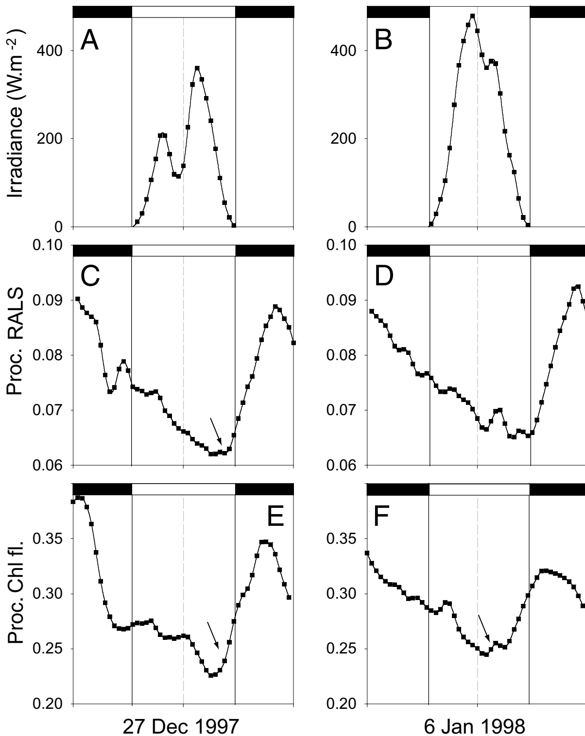
Fig. 9. Comparison between two selected days (December 27, 1997 and January 6, 1998) for light irradiance (A, B), Prochlorococcus RALS (C, D) and Chl fluorescence (E, F). All data were smoothed using a low-pass filter removing frequencies above 0.5 \text{ h}^{-1} with the equation: y_i = a_6 \cdot x_{i-6} + \dots + a_0 \cdot x_i + \dots + a_6 \cdot x_{i+6} with a_0 = 0.303 , a_1 = 0.217 , a_2 = 0.055 , a_3 = 0.033 , a_4 = 0.025 , a_5 = 0.013 , a_6 = 0.005 , and where x_i and y_i are the original and smoothed data, respectively, at time t_i .
