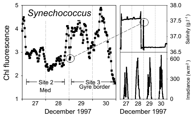
Fig. 10. Pattern recorded for Chl fluorescence of Synechococcus cells (smoothed data obtained as on Figure 9) between December 27 and 30, 1997 in association with salinity and irradiance fluctuations. The two circles are drawn to symbolize the strong correlation between hydrological conditions and chlorophyll fluorescence of the cells.
