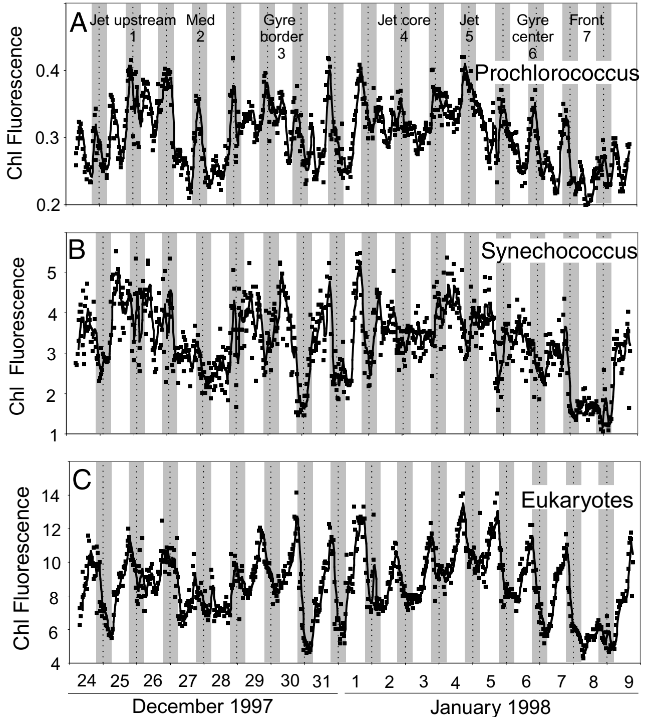
Fig. 8. Red chlorophyll (Chl) fluorescence of Prochlorococcus (A), Synechococcus (B) and picoeukaryotes (C) sampled every 30 min between December 24, 1997 and January 9, 1998. Curves and symbols as on Figure 5.
