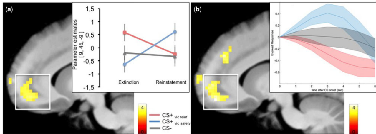
Fig. 5. (a) Change in vmPFC activity from extinction to reinstatement testing displayed for all CSs separately (b). Mean estimated evoked responses (arbitrary units) within the vmPFC during Reinstatement test scaled to the response at onset of each CS. Shaded areas represent SEM. T-values are superimposed on a normalized average structural image. fMRI display threshold: P < 0.005 , uncorrected for illustrative purposes.
